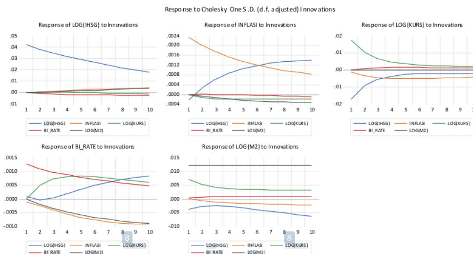
Figure 1. Impulse response function (IRF) results
