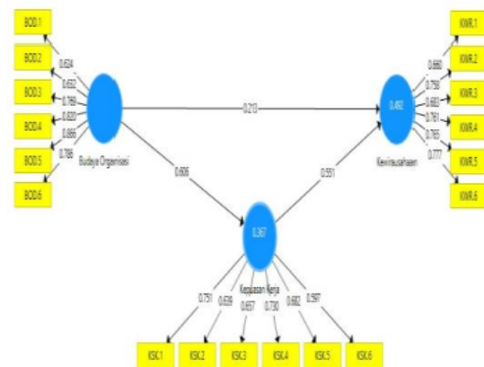
Gambar 1. Hasil Model Internal
